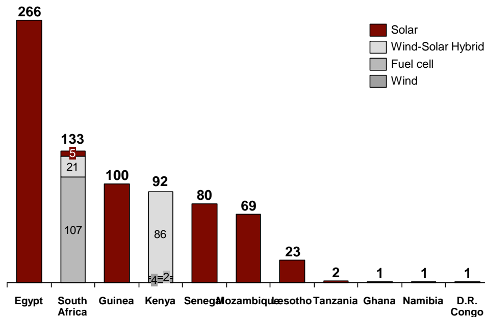
Figure 26: Base Stations Powered by Alternative Renewable Energy Sources 57
